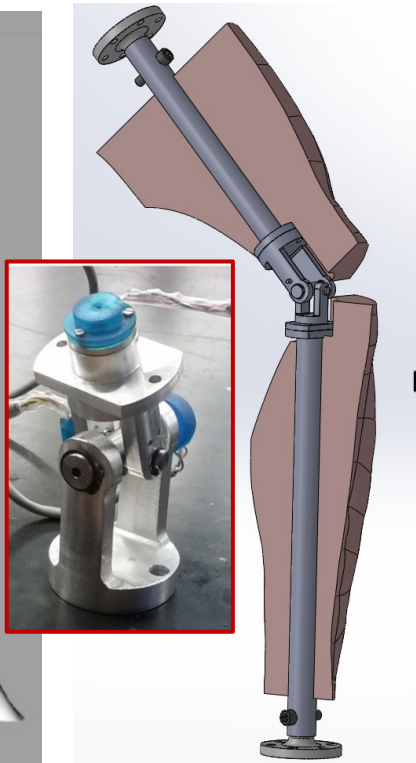
Instrumented Cardan Joint
